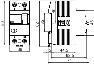
Figure 1 – Overall and installation dimensions of 2-polar VDs
